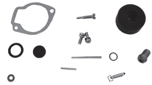
Carb Kit All 2 HP Part No: 6A1-W0093-01
