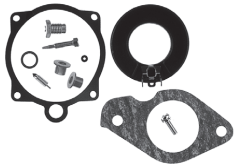
Carb Kit 25-30 HP 84-97 Part No: 689-W0093-02
