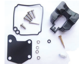
C arb Kit 9.9-15 HP 96-Up Part No: 63V-W0093-00
