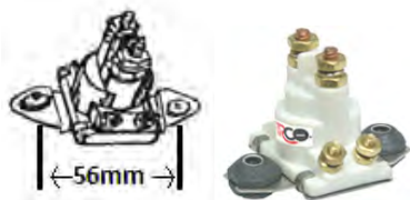
Starter Relay
