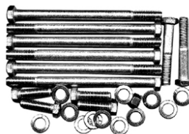
Powerhead Mounting Bolts Stainless Steel Fits All V-6 Loopers 6 x 5-1/2" Bolts (3/8" x 16) 2 x 2-1/4" Bolts (3/8" x 16) 4 x 1-1/4" Bolts (3/8" x 16) 2 x 1-1/4" Bolts (5/16" x 18) 3 x Nuts (5/16" x 24) 5 x 5/16" Lock Washer 12 x 3/8" Lock Washer Part No: 353
