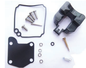
Carb Kit 9.9-15 HP 96-Up Part No: 63V-W0093-00
